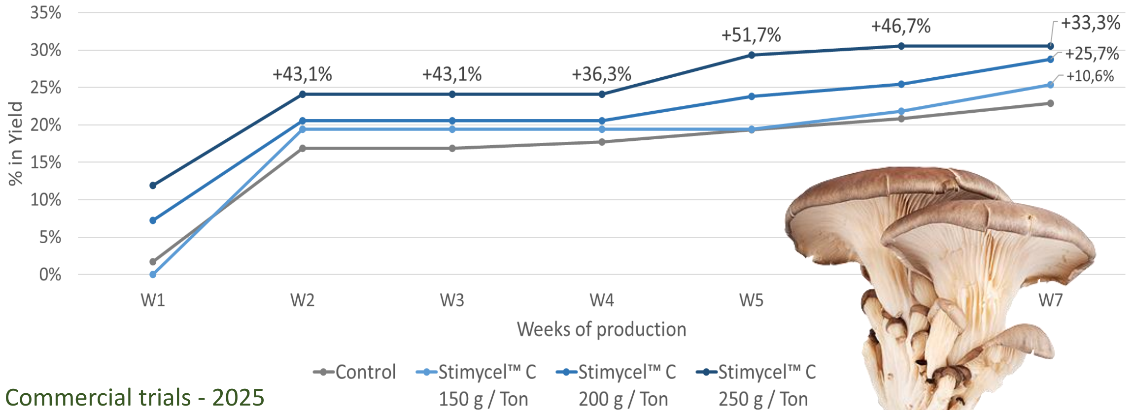
Yields of Oysters (strain M2191) produced on pasteurized substrate with addition of Stimycel™ C
